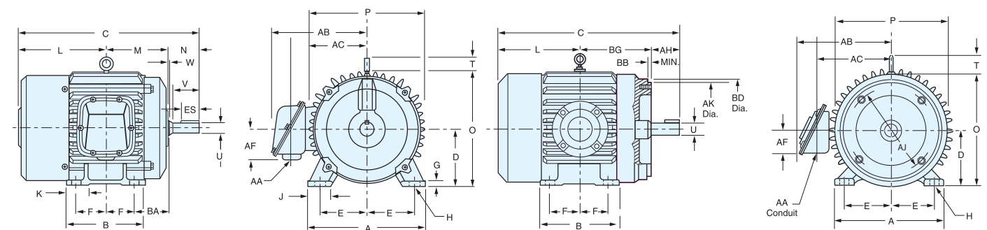
NEMA EXPLOSION-PROOF, 158 SERIES, RIGID MOUNT DIMENSIONS (INCHES)
